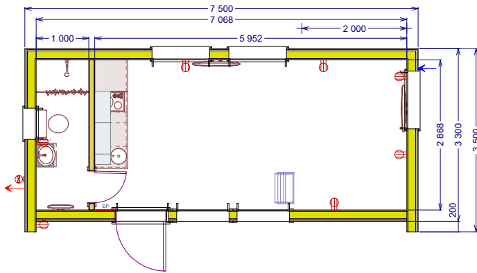
Plan 1
